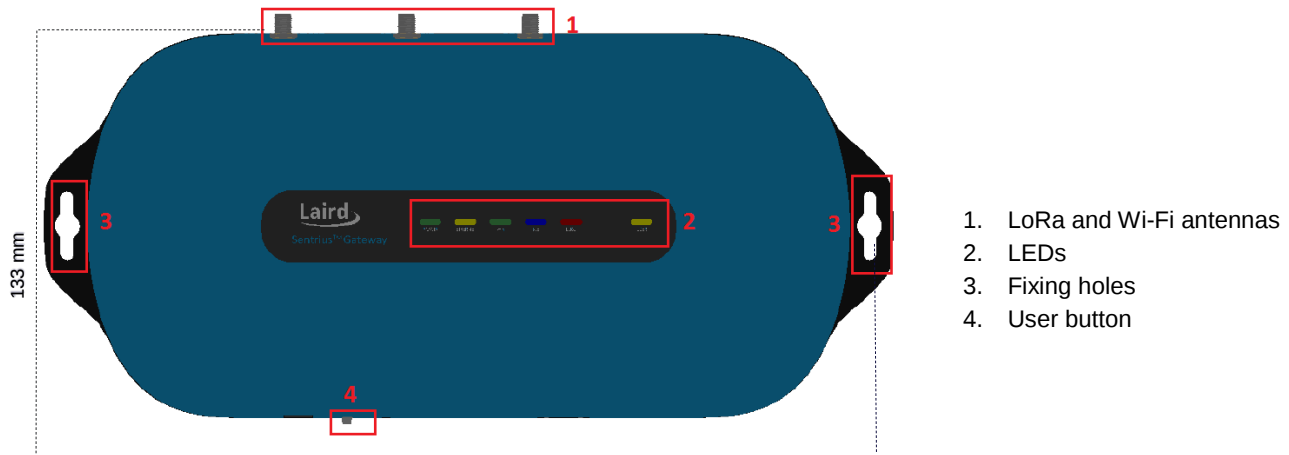
Figure 1: Top of the Sentrius™ RG1xx gateway
